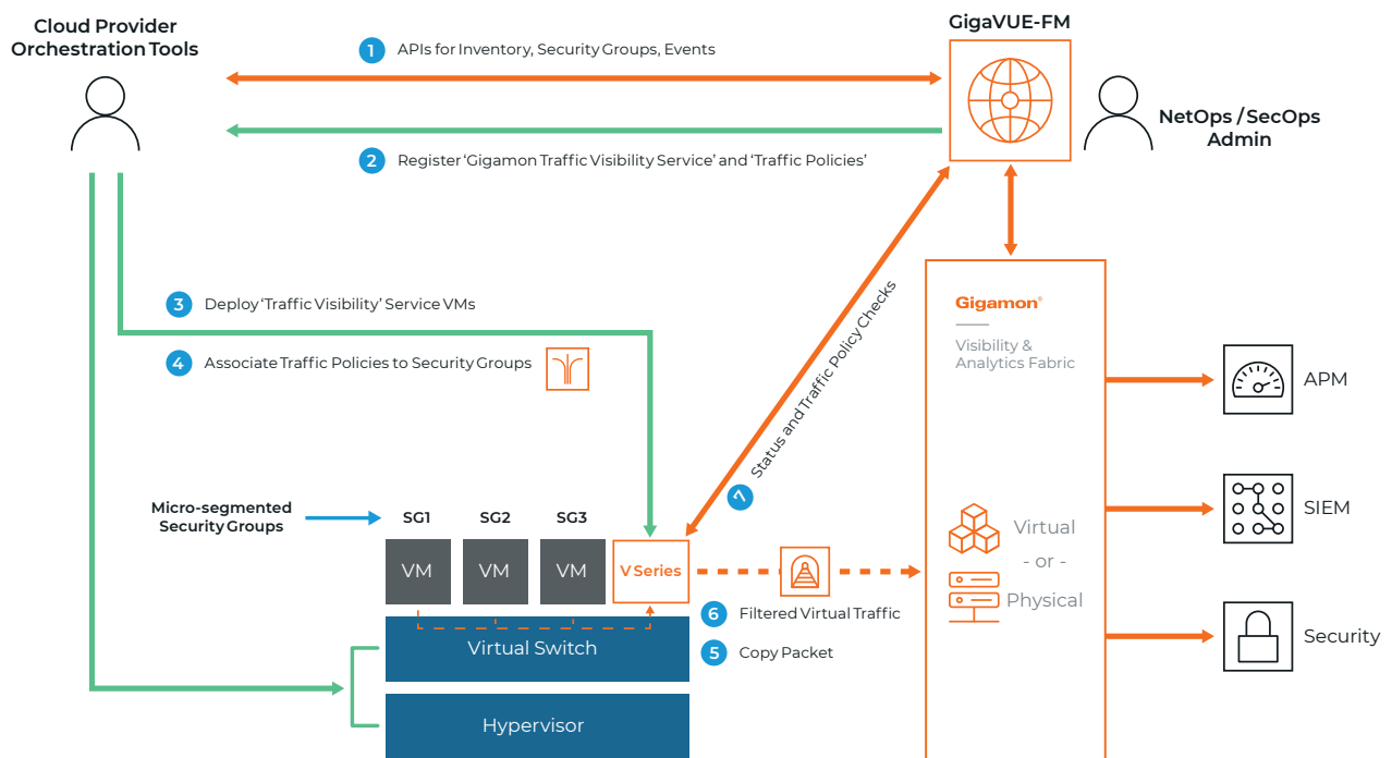
Figure 2: Straightforward seven-step process for provisioning, configuration, and monitoring.
